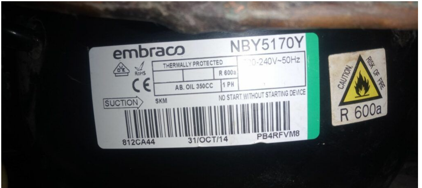
File Pdf: NBY5170Y, Compressor, 1/4 HP, 1ph 220-240V/50Hz, R600a, 15kg, High Back Pressure, HBP, Commercial Refrigeration, Embraco
